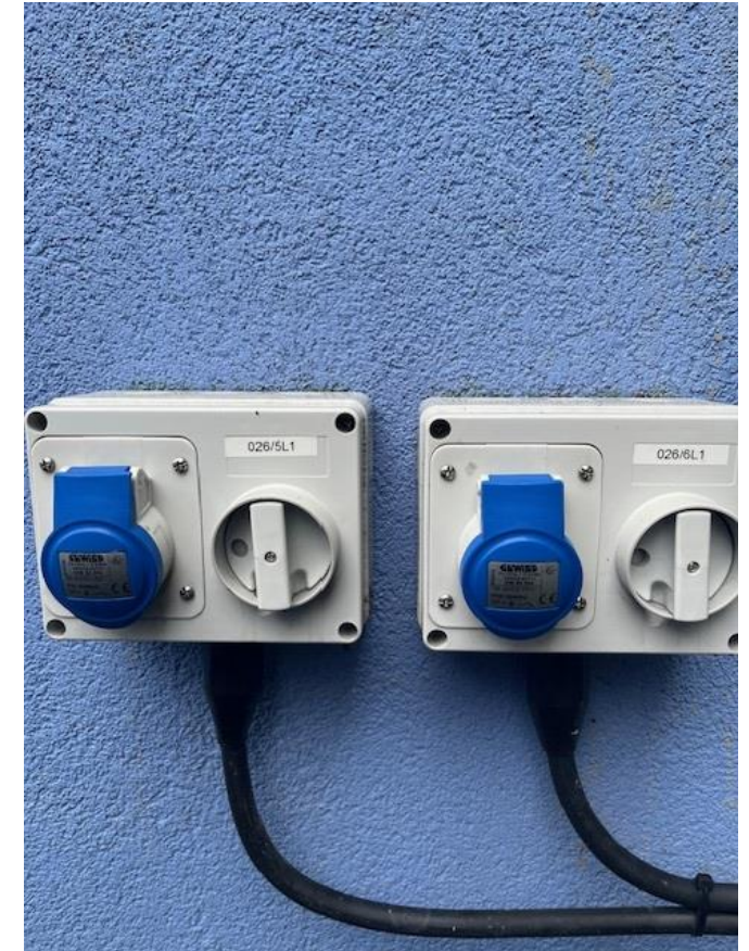
2 x commando style plugs
