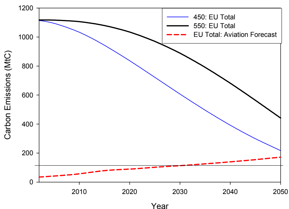
Figure 7: Contraction and convergence profiles to meet 450ppmv and 550ppmv carbon dioxide concentrations for the EU25 nations compared with projected aviation emissions for those nations. Emissions profile in black thick solid line for 550ppmv, blue (thin) solid for the 450ppmv and dashed for the forecasted aviation emissions for the EU25 nations.
