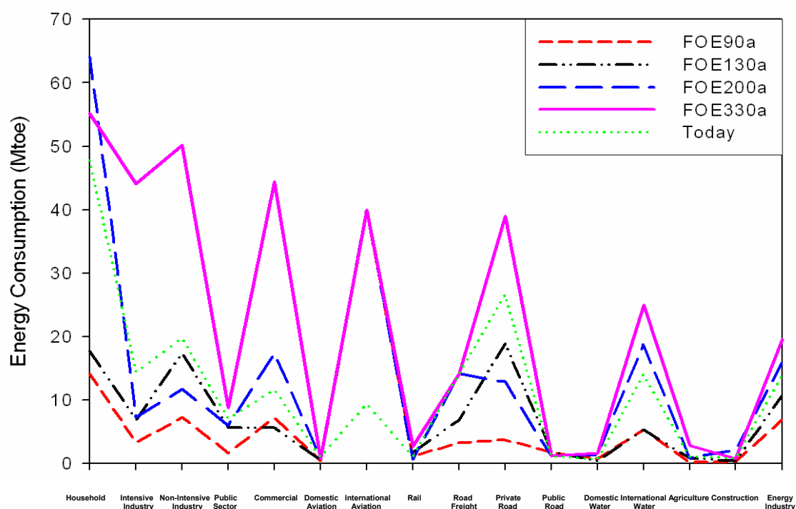
Figure 10: Energy consumption profiles for the four FOE scenarios that meet the UK government's 60% carbon reduction target. The profile for today is also shown.
