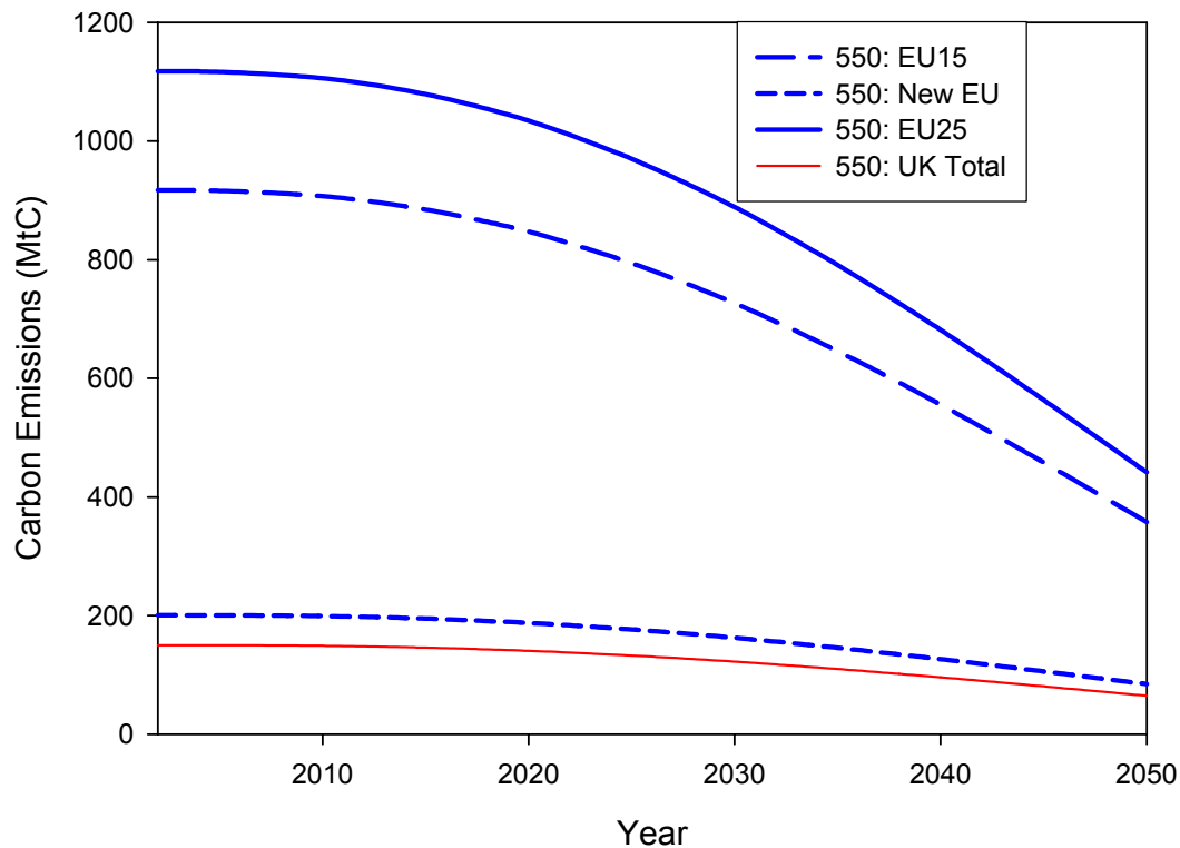
Figure 3: Contraction and convergence profile to meet a 550ppmv carbon dioxide concentration. The emissions profile shown as a blue solid line (thick solid line for black and white) is for the whole of the EU, the long dashed line is for the EU15 nations, short dashed line for New EU nations (accession nations) and in red (thin solid) for the UK.
