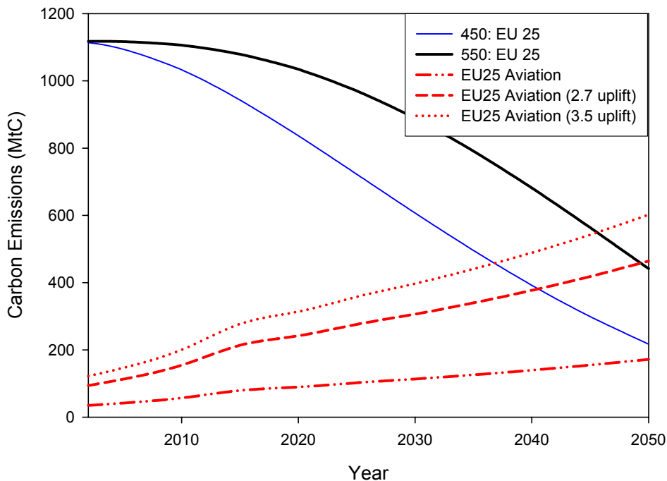
Figure 8: Contraction and convergence profiles to meet 450ppmv and 550ppmv carbon dioxide concentrations for the EU25 nations compared with their projected aviation emissions with no uplift, uplifted by 2.7 and uplifted by 3.5. Emissions profile in black thick solid line for 550ppmv, blue (thin) solid for the 450ppmv, dash-dot-dot for no uplift, short dash for an uplift of 2.7, and dotted for 3.5 uplift.
