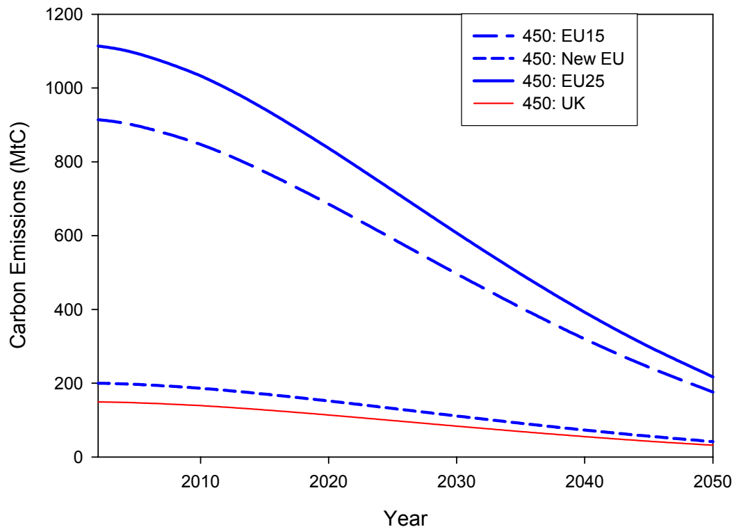
Figure 4: Contraction and convergence profile to meet a 450ppmv carbon dioxide concentration. Emissions profile in blue (thick) solid line for the whole of the EU, long dash for the EU15 nations, short dash for New EU nations and in red (thin) for the UK.
