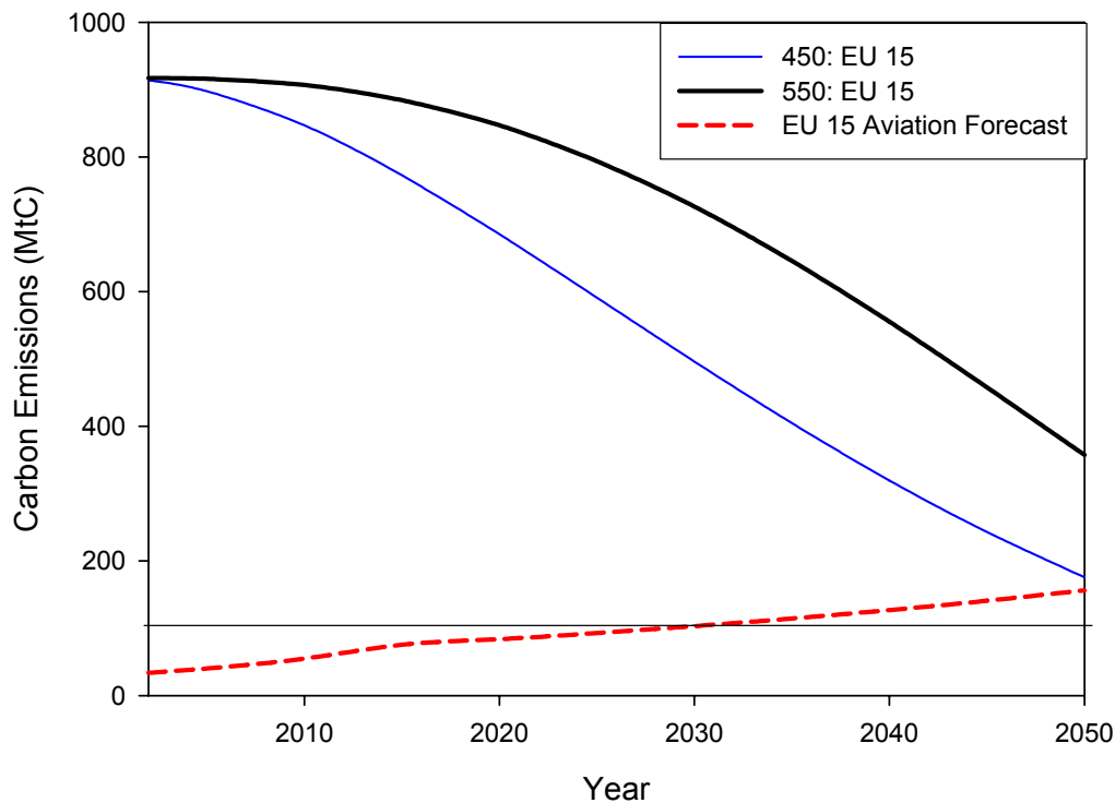
Figure 5: Contraction and convergence profiles to meet 450ppmv and 550ppmv carbon dioxide concentrations for the EU15 nations, compared with projected aviation emissions for those nations. Emissions profile in thick black solid line for 550ppmv, blue (lighter) solid for the 450ppmv and dashed for the forecasted aviation emissions for the EU15 nations.
