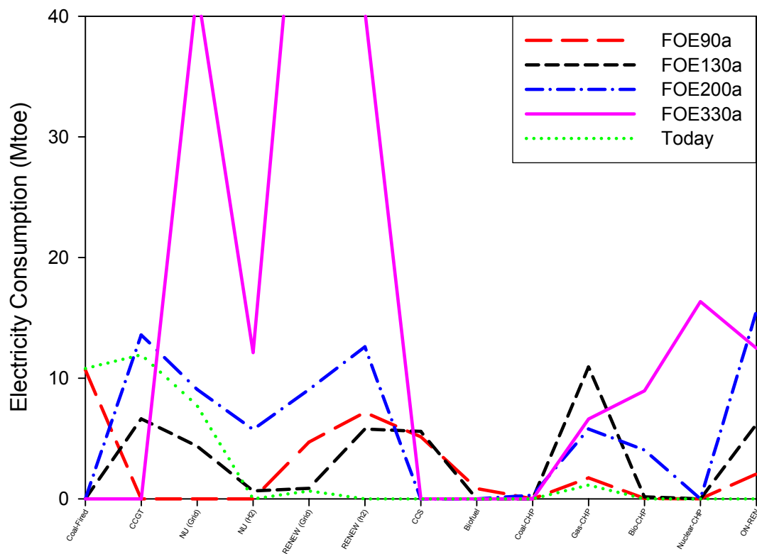
Figure 12: Electricity demand profiles for the four FOE scenarios that meet the UK government's 60% carbon reduction target, in terms of the source of the supply. The profile for today is also shown. Coal-fired, CCGT (combined-cycle gas turbines), NU (Grid) (nuclear), RENEW (Grid) (renewables), CCS (coal-fired power with carbon capture and storage) and biofuel are all sources for the national grid. NU (H2) (nuclear), RENEW (H2) (renewables) are electricity required for hydrogen production, Coal-CHP, Gas-CHP, Bio-CHP and Nuclear-CHP are the different combined heat and power sources, and ON-REN are on-site renewables.
