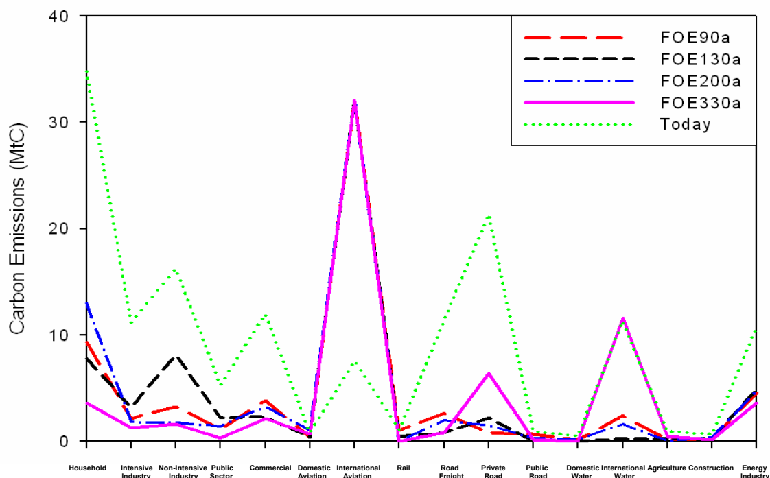
Figure 11: Carbon emission profiles for the four FOE scenarios that meet the UK government's 60% carbon reduction target. The profile for today is also shown.
