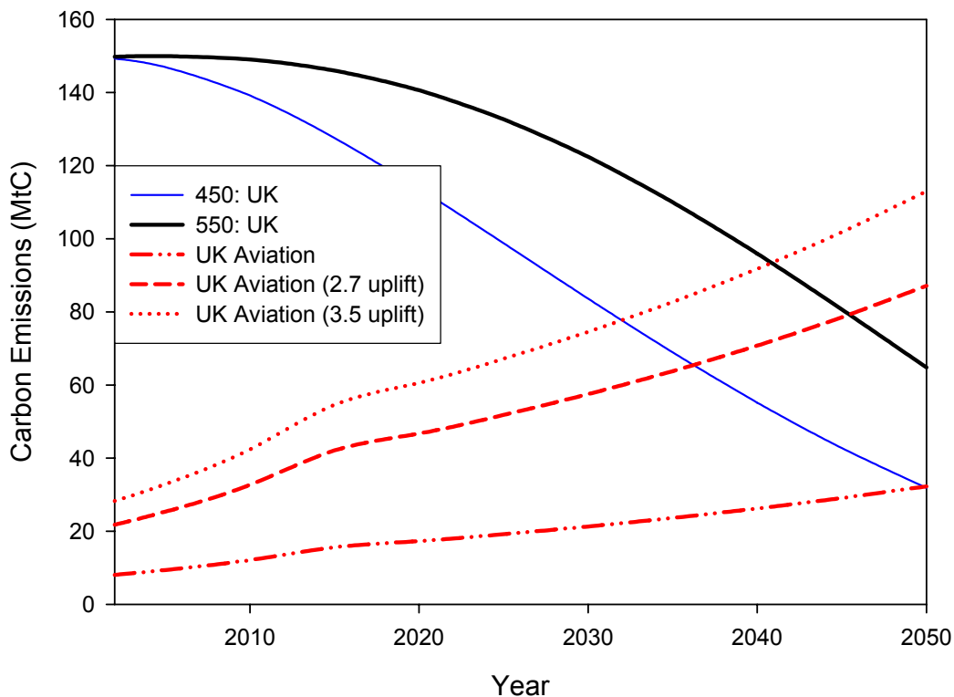
Figure 9: Contraction and convergence profiles to meet 450ppmv and 550ppmv carbon dioxide concentrations for the UK compared with the UK's projected aviation emissions with no uplift, uplifted by 2.7 and uplifted by 3.5. Emissions profile in black thick solid line for 550ppmv, blue (light) solid for the 450ppmv, dash-dot-dot for no uplift, short dash for an uplift of 2.7, and dotted for 3.5 uplift.
