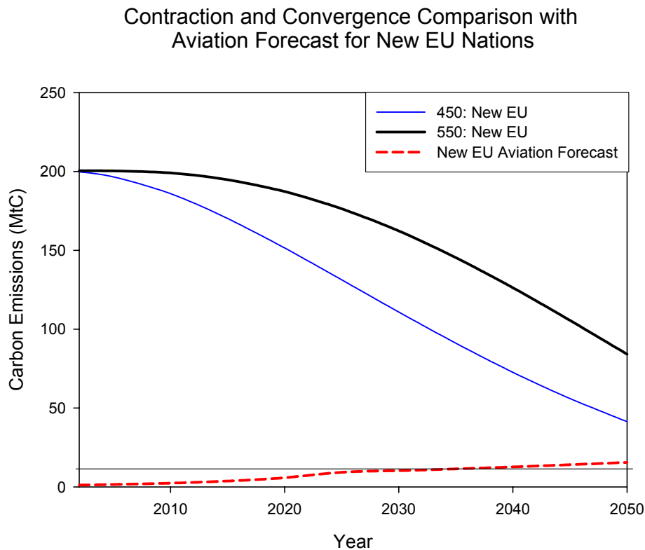
Figure 6: Contraction and convergence profiles to meet 450ppmv and 550ppmv carbon dioxide concentrations for the New EU nations compared with projected aviation emissions for those nations. Emissions profile in black thick solid line for 550ppmv, blue (thin) solid for the 450ppmv and dashed for the forecasted aviation emissions for the New EU nations.
