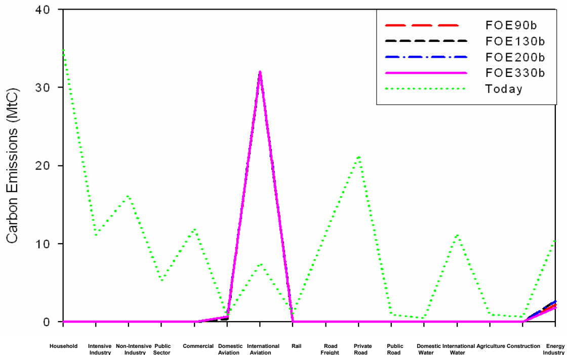
Figure 14: Carbon emission profiles for the four FOE scenarios that try to achieve a carbon dioxide concentration that stabilises at 450ppmv. The profile for today is also shown.
