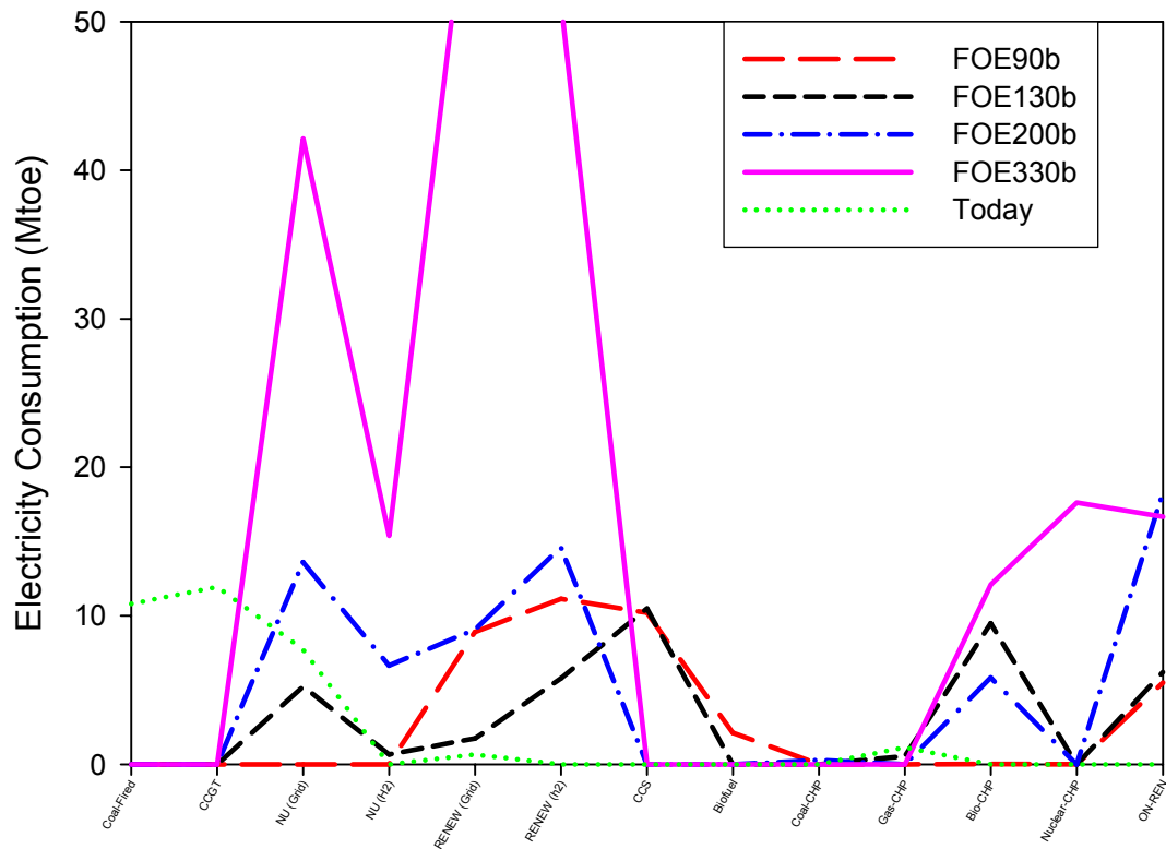
Figure 15: Electricity demand profiles for the four FOE scenarios that reach a level that attains a carbon dioxide stabilisation of 450ppmv, in terms of the source of the supply. The profile for today is also shown. Coal-fired, CCGT (combined-cycle gas turbines), NU (Grid) (nuclear), RENEW (Grid) (renewables), CCS (coal-fired power with carbon capture and storage) and biofuel are all sources for the national grid. NU (H2) (nuclear), RENEW (H2) (renewables) are electricity required for hydrogen production, Coal-CHP, Gas-CHP, Bio-CHP and Nuclear-CHP are the different combined heat and power sources, and ON-REN are on-site renewables.
