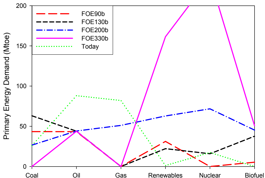
Figure 16: Primary energy demand profiles for the four FOE scenarios that attain a carbon dioxide stabilisation level of 450ppmv, in terms of primary fuels. The profile for today is also shown.
